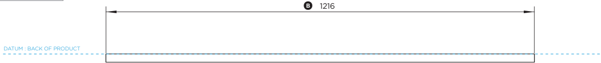
PLAN VIEW
