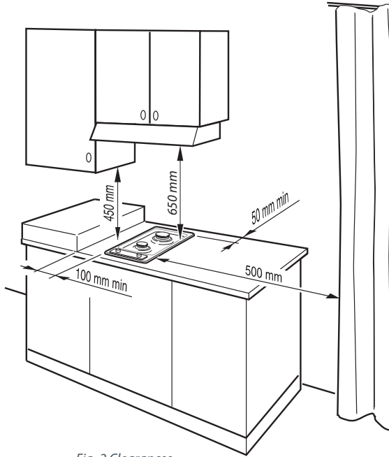
Fig. 2 Clearances
