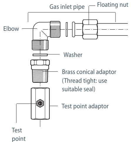
Fig. 7 LPG connection
