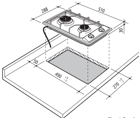
Fig. 1 Product and cutout dimensions
