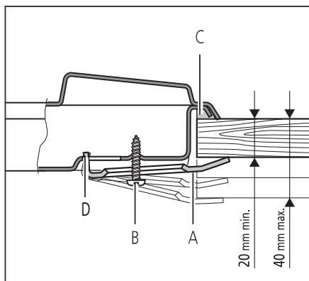
Fig. 5 Fastening the cooktop
