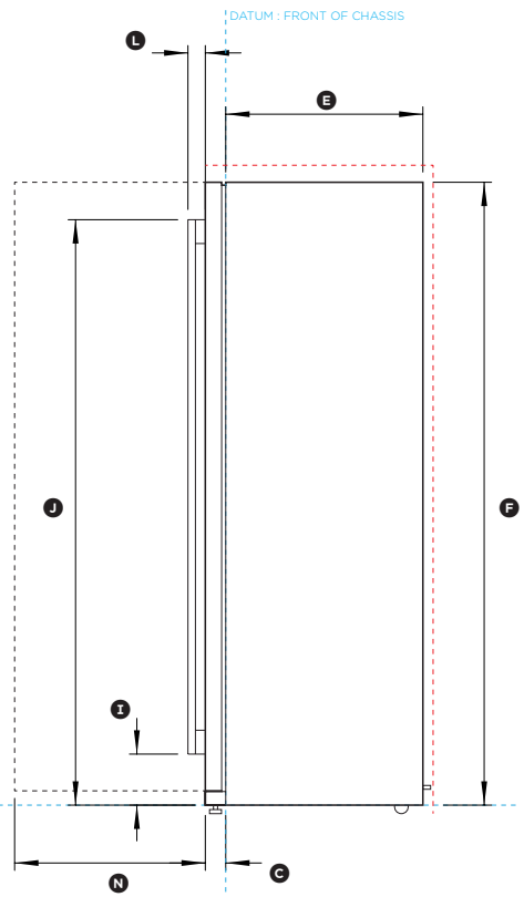
PROFILE VIEW
