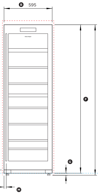
FRONT VIEW
