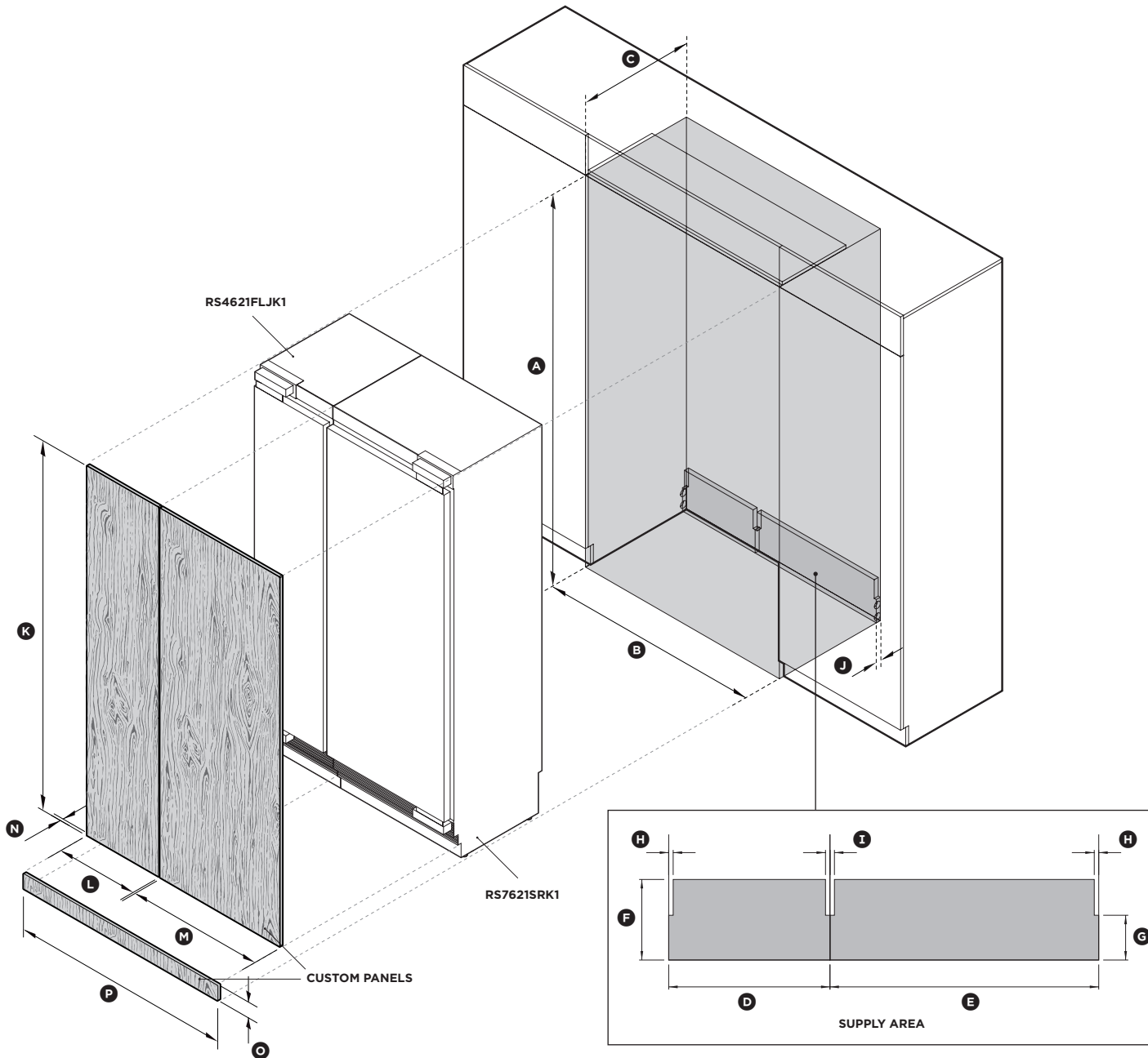
ISO VIEW OF 1219mm CAVITY (457mm + 762mm)
