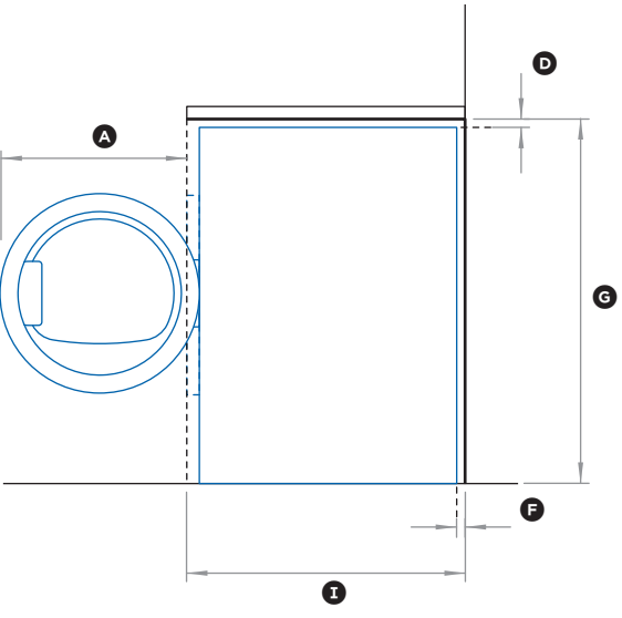
PROFILE VIEW DRYER
