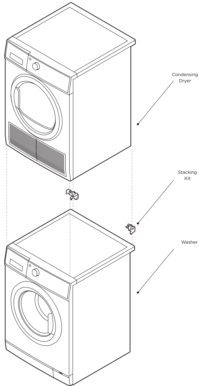
EXPLODED ISO VIEW
