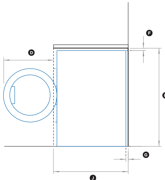
PROFILE VIEW
