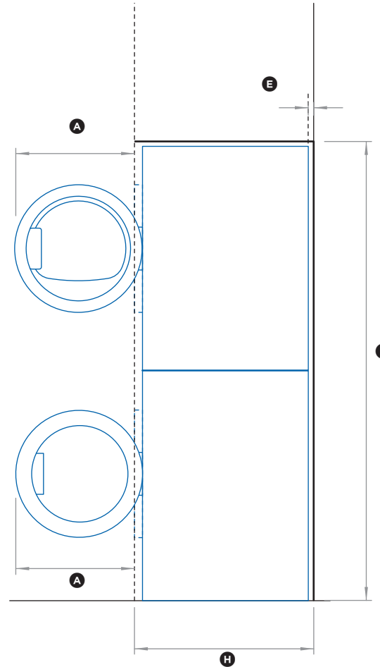
PROFILE VIEW
