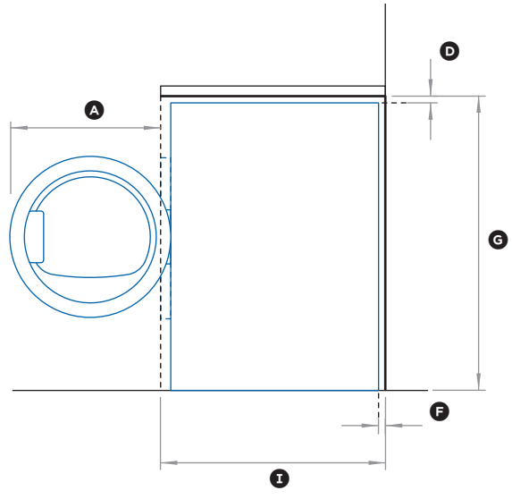
PROFILE VIEW DRYER
