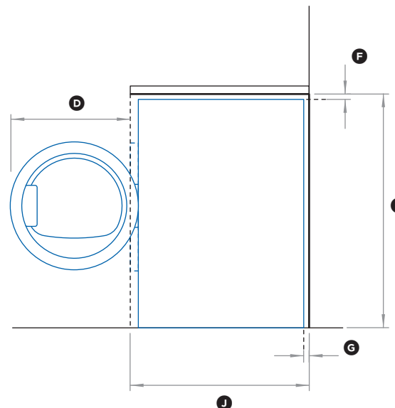
PROFILE VIEW
