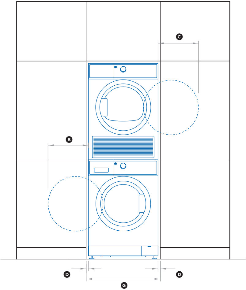
FRONT VIEW
