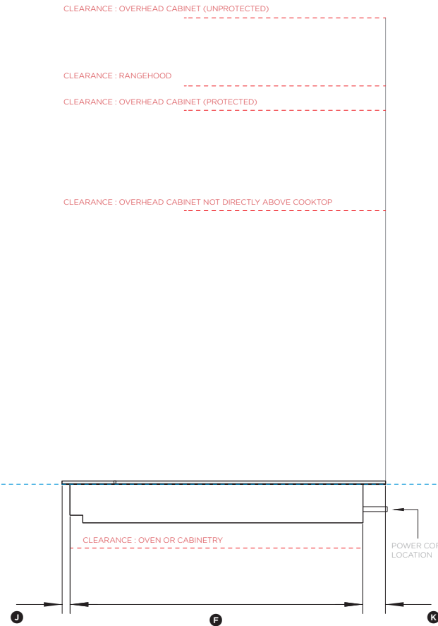
PROFILE VIEW
