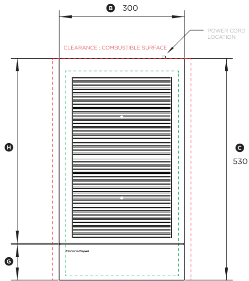
PLAN VIEW
