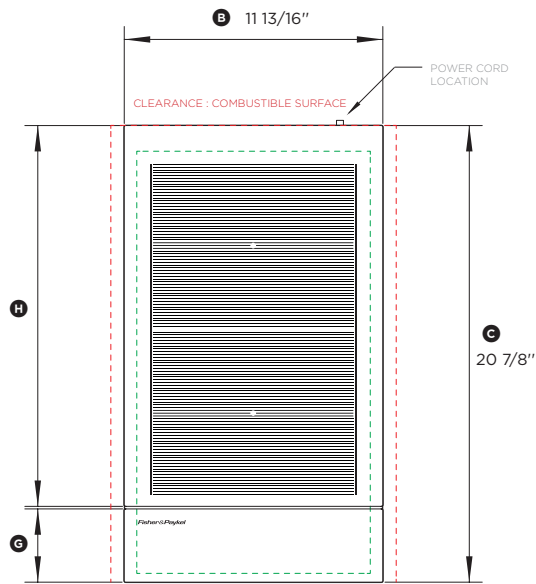
PLAN VIEW
