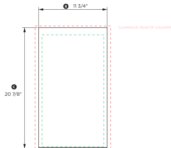
PLAN VIEW
