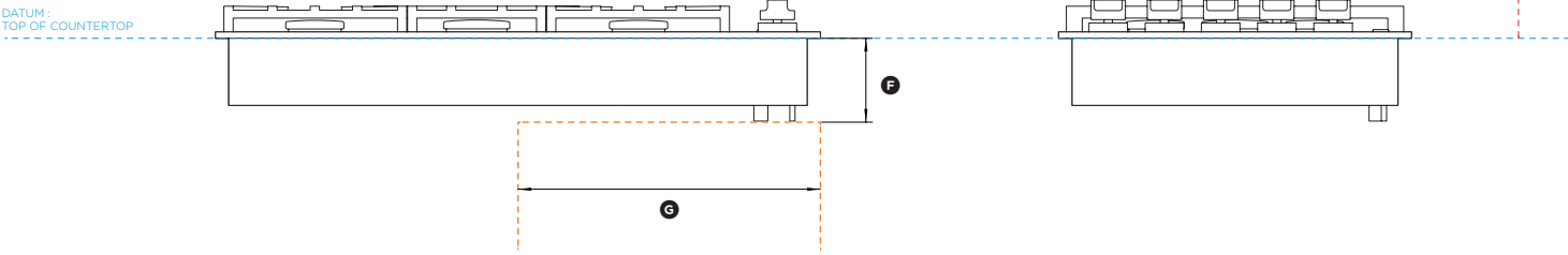
FRONT VIEW
