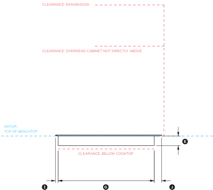
PROFILE VIEW
