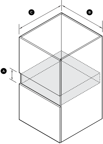
ISO VIEW
