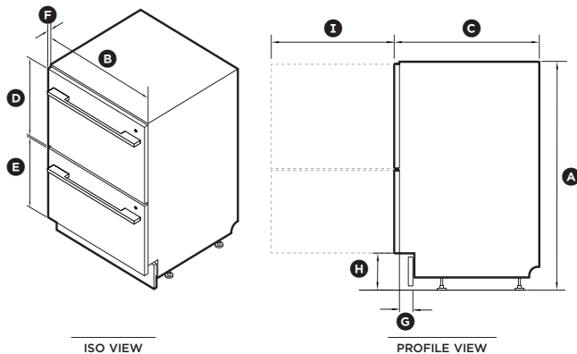
ISO VIEW
