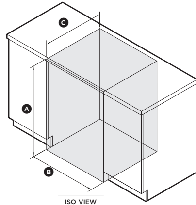
ISO VIEW
